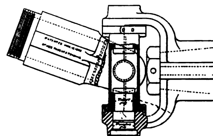
MUTUAL SIMPLE UNIVERSAL JOINT.
